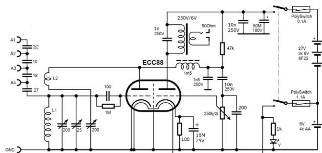
SW Audion OK1DPX 2019
